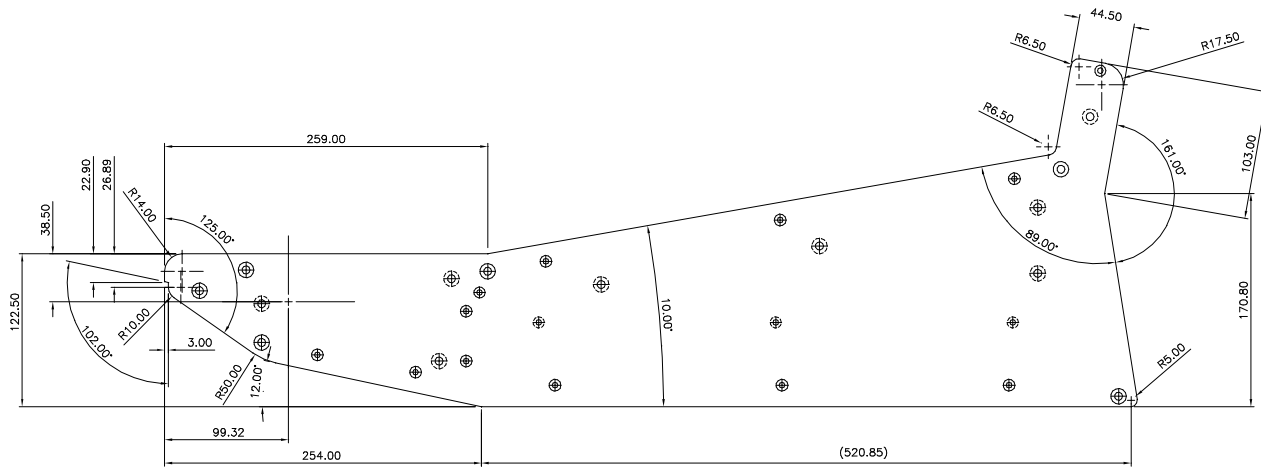
PROFILE DIMENSIONS
