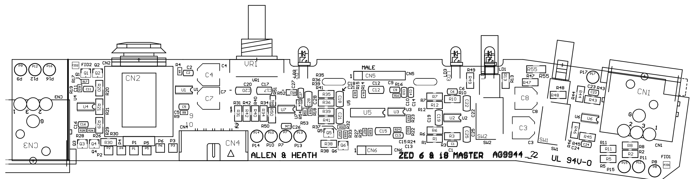
ALLEN & HEATH ZED 6 MASTER PCB AG9944 2
