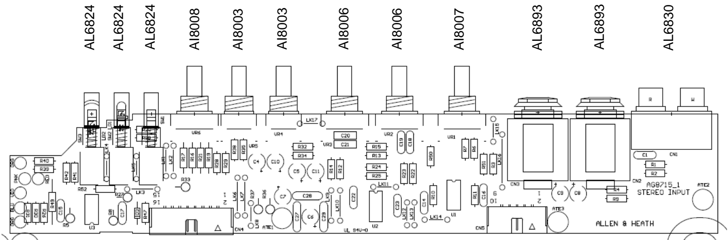
004-297 Stereo IP 2
