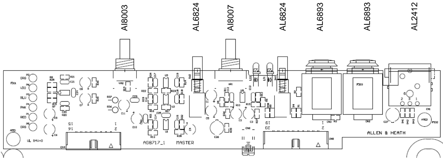
004-299 Master
