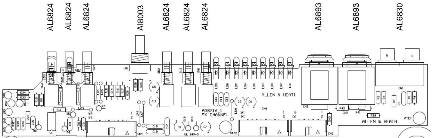
004-298 Effects
