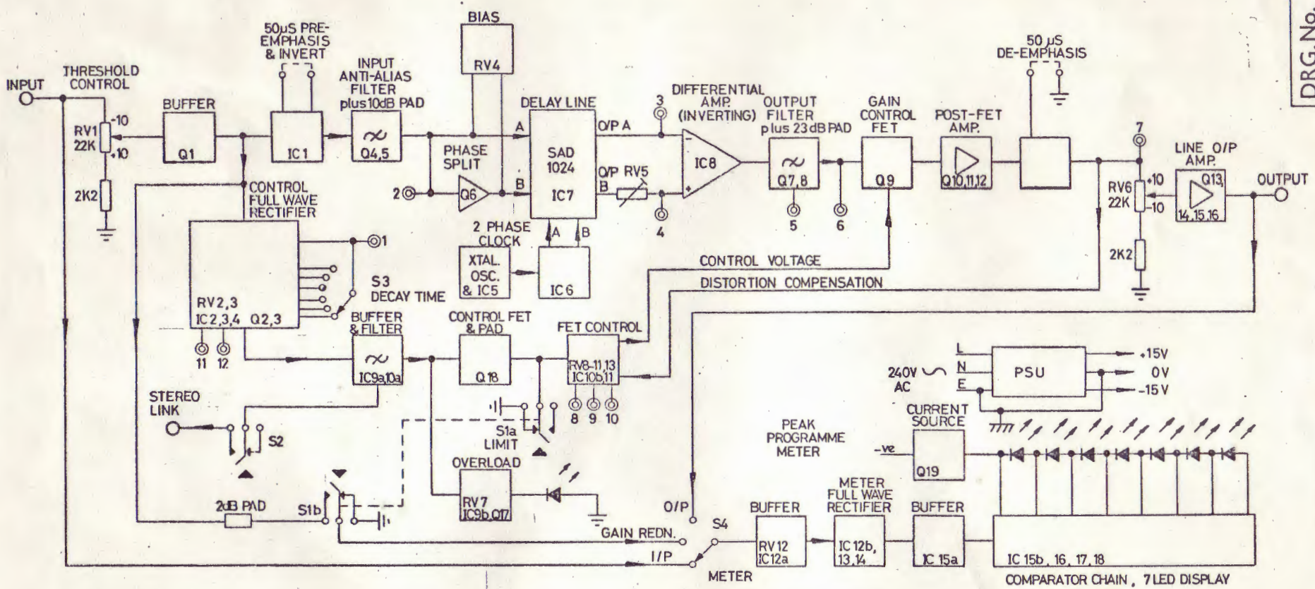
FEED FORWARD DELAY LIMITER BLOCK DIAGRAM
